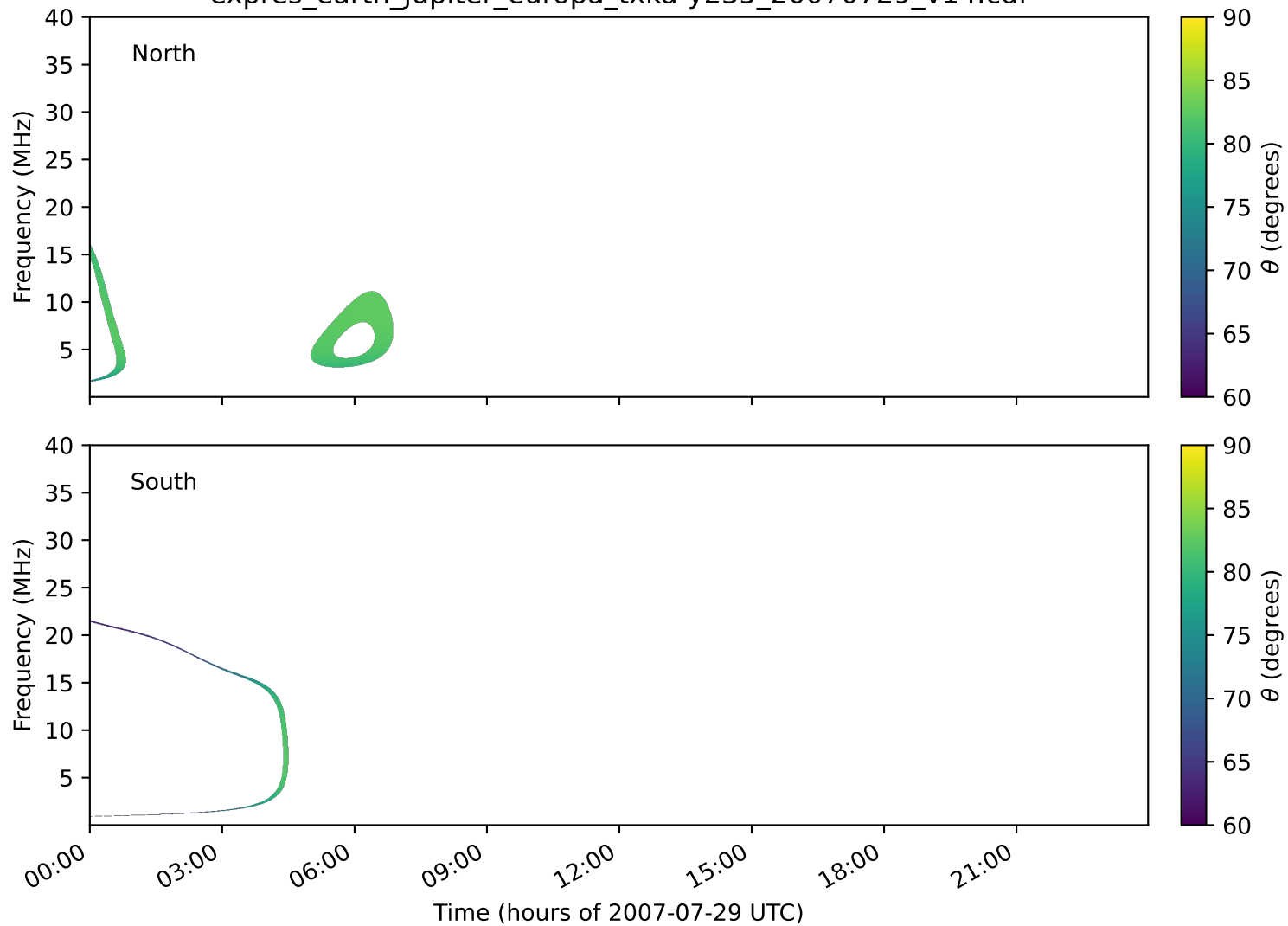
expres_earth_jupiter_europa_txka-y235_20070729_v14.cdf
