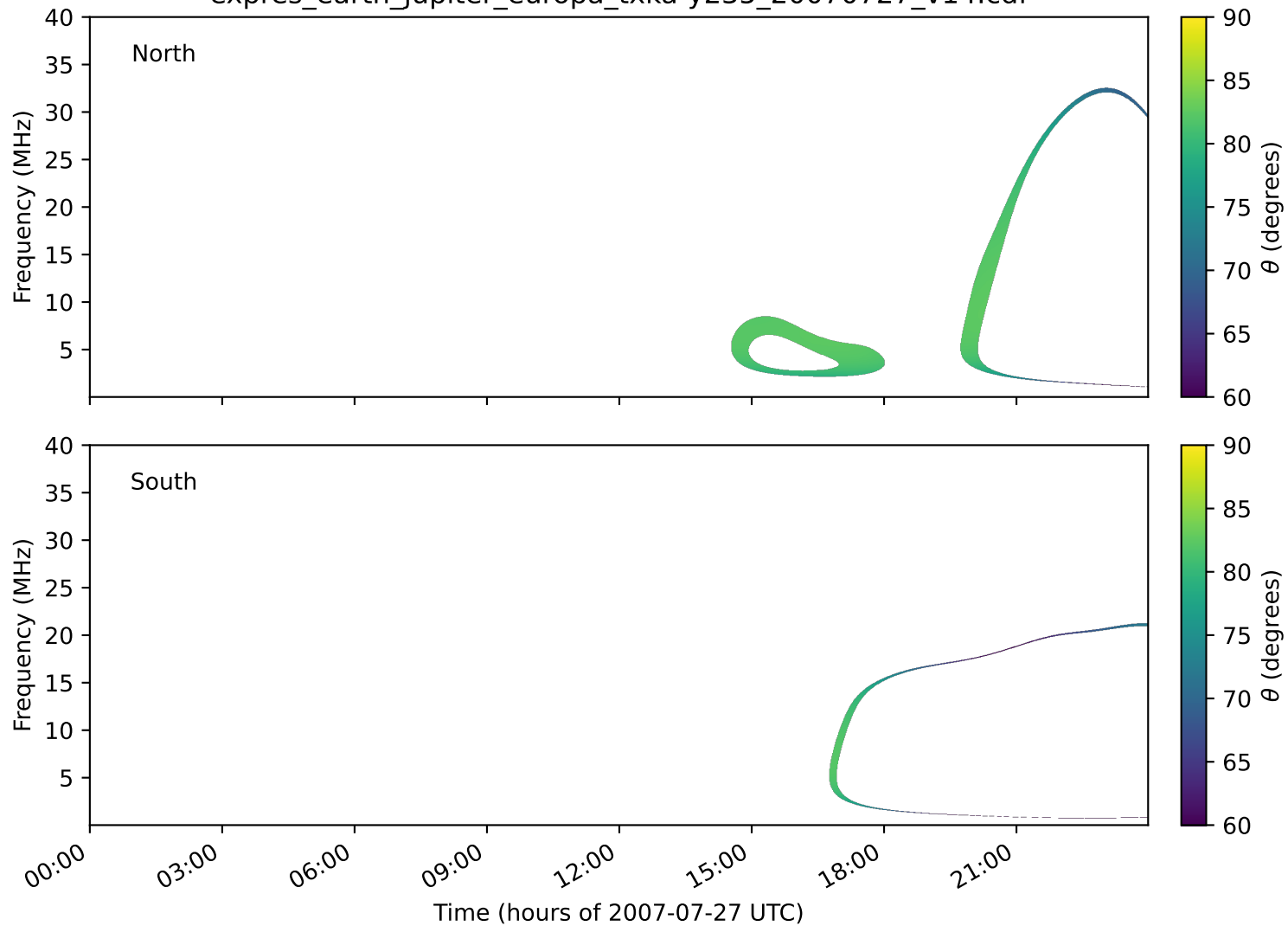
expres_earth_jupiter_europa_txka-y235_20070727_v14.cdf
