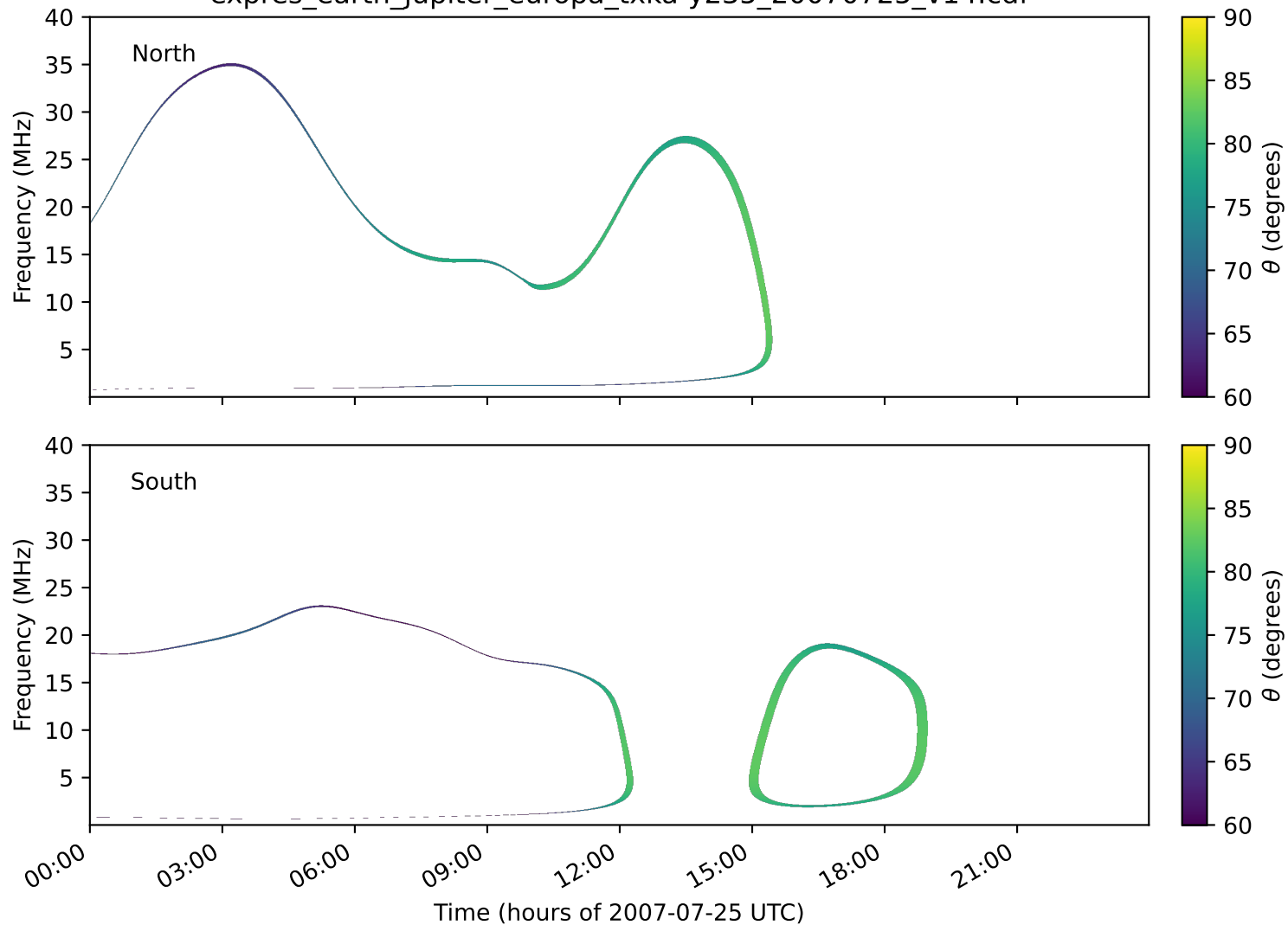
expres_earth_jupiter_europa_txka-y235_20070725_v14.cdf
