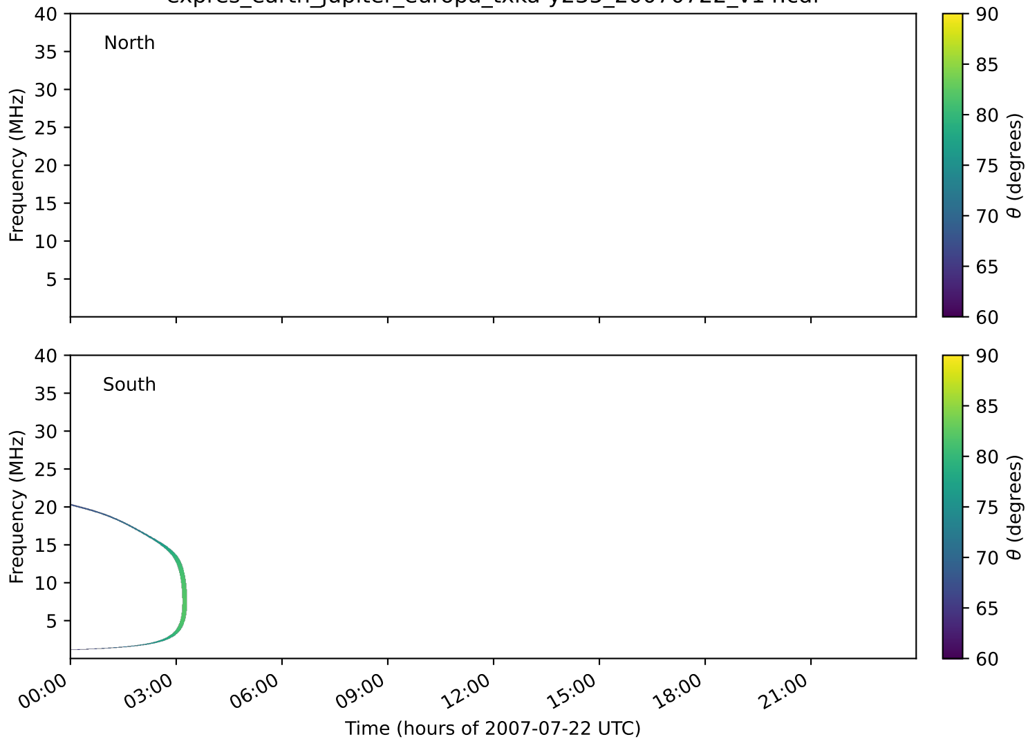
expres_earth_jupiter_europa_txka-y235_20070722_v14.cdf
