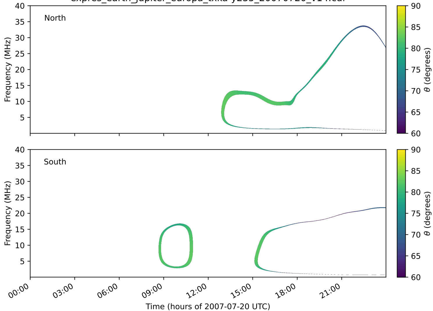
expres_earth_jupiter_europa_txka-y235_20070720_v14.cdf
