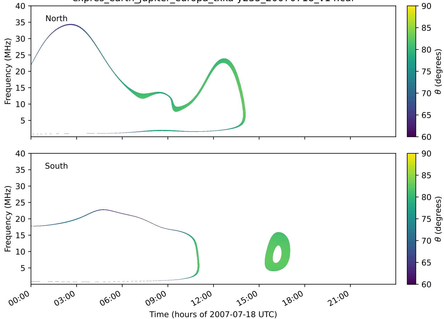
expres_earth_jupiter_europa_txka-y235_20070718_v14.cdf
