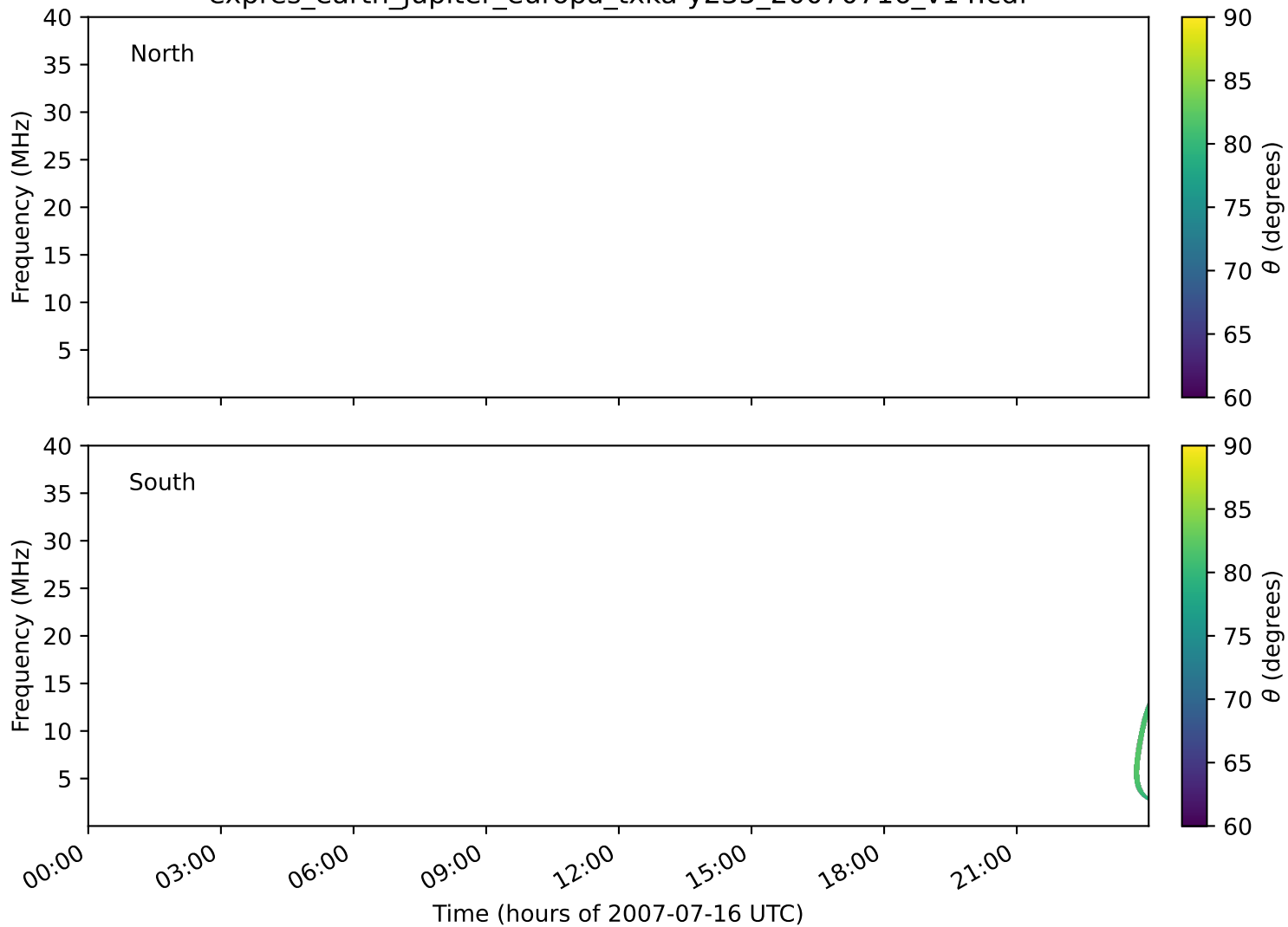
expres_earth_jupiter_europa_txka-y235_20070716_v14.cdf
