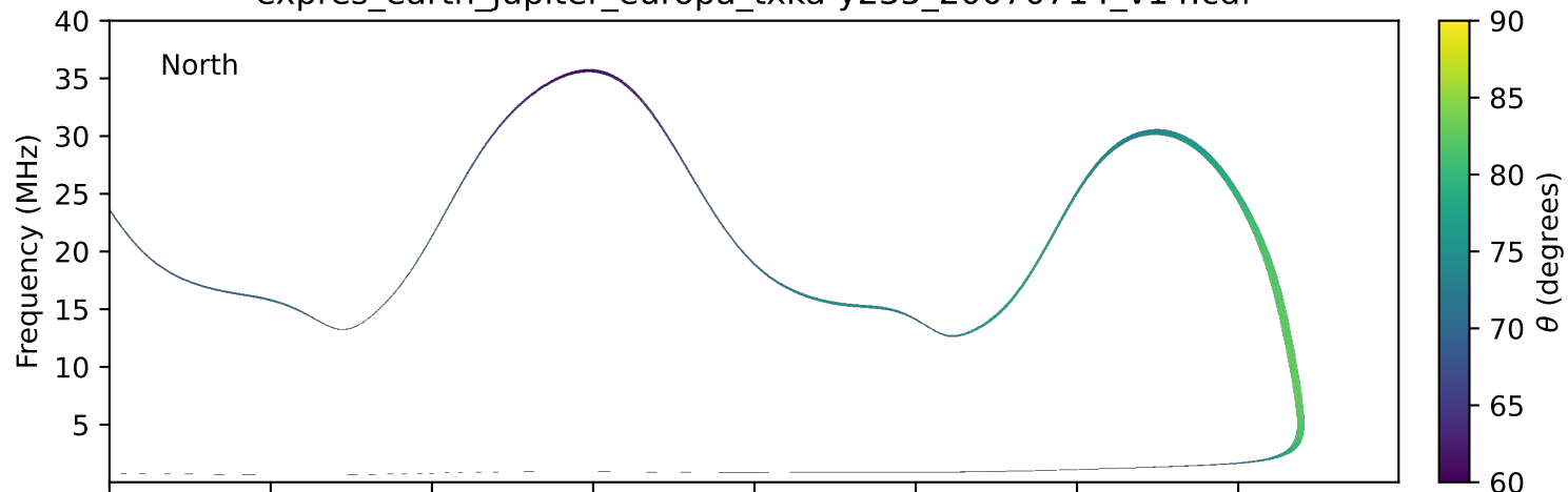
expres_earth_jupiter_europa_txka-y235_20070714_v14.cdf
