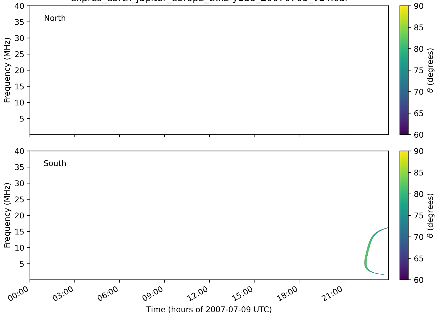
expres_earth_jupiter_europa_txka-y235_20070709_v14.cdf
