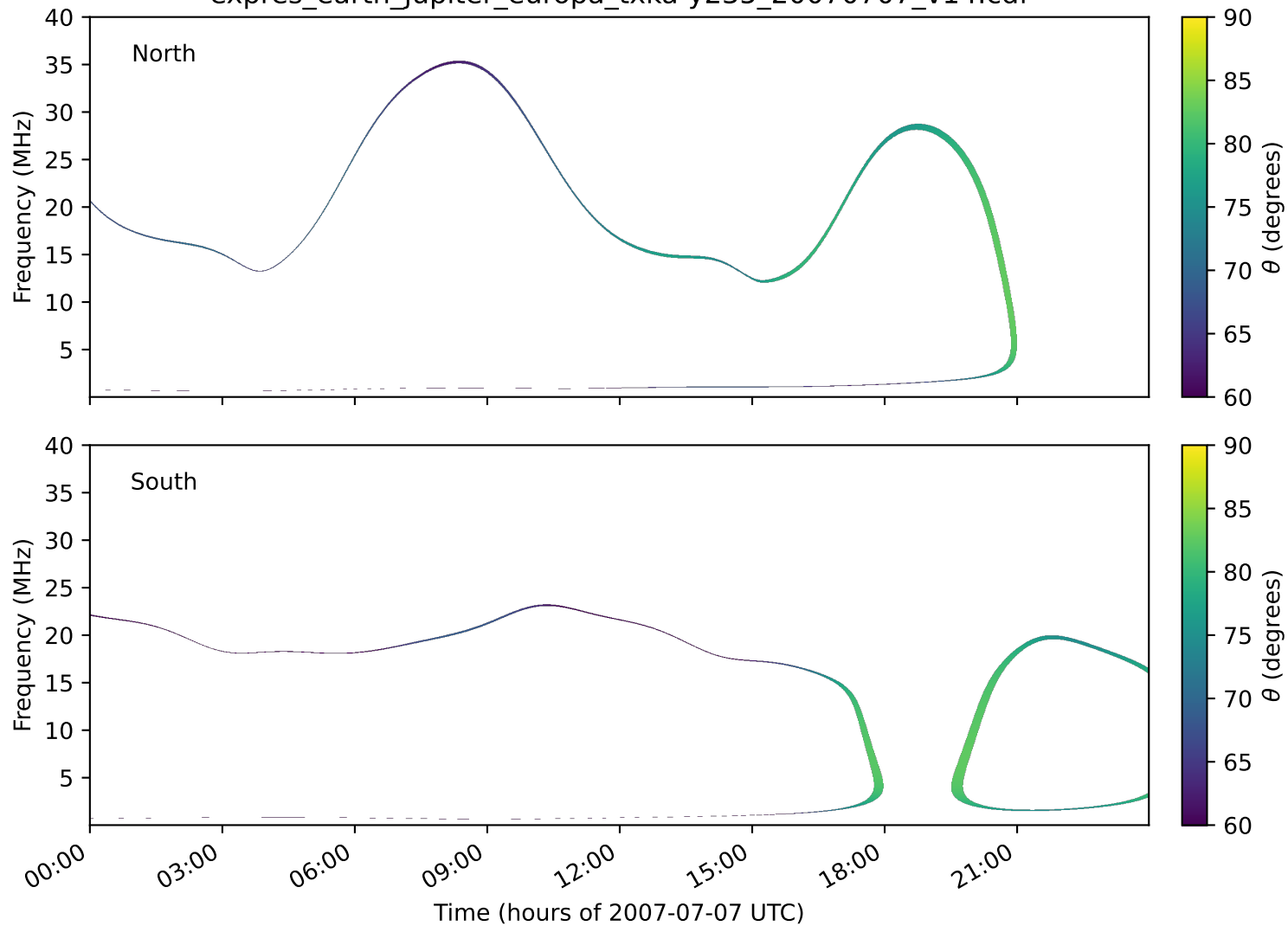
expres_earth_jupiter_europa_txka-y235_20070707_v14.cdf
