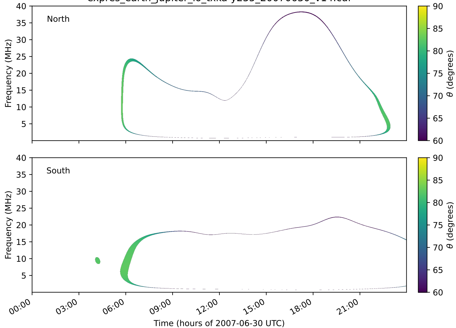
expres_earth_jupiter_io_txka-y235_20070630_v14.cdf
