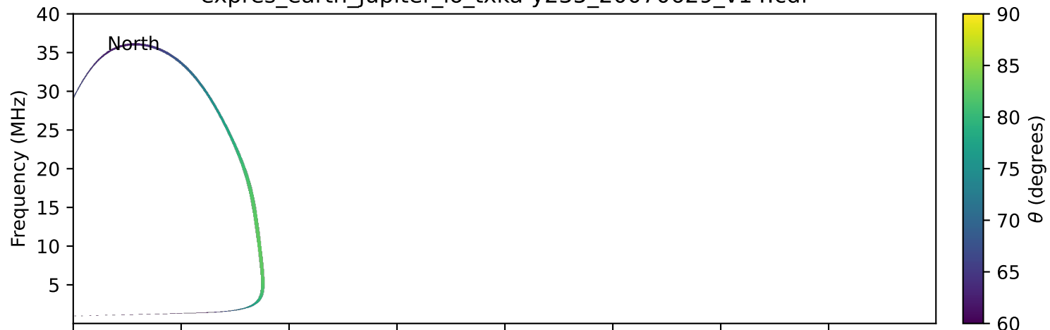
expres_earth_jupiter_io_txka-y235_20070629_v14.cdf
