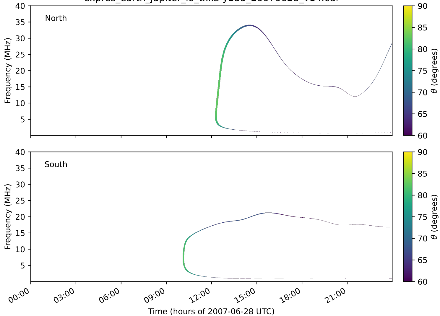
expres_earth_jupiter_io_txka-y235_20070628_v14.cdf
