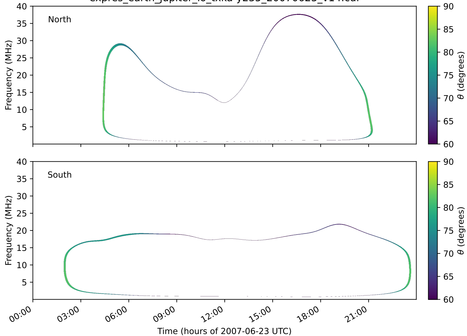
expres_earth_jupiter_io_txka-y235_20070623_v14.cdf
