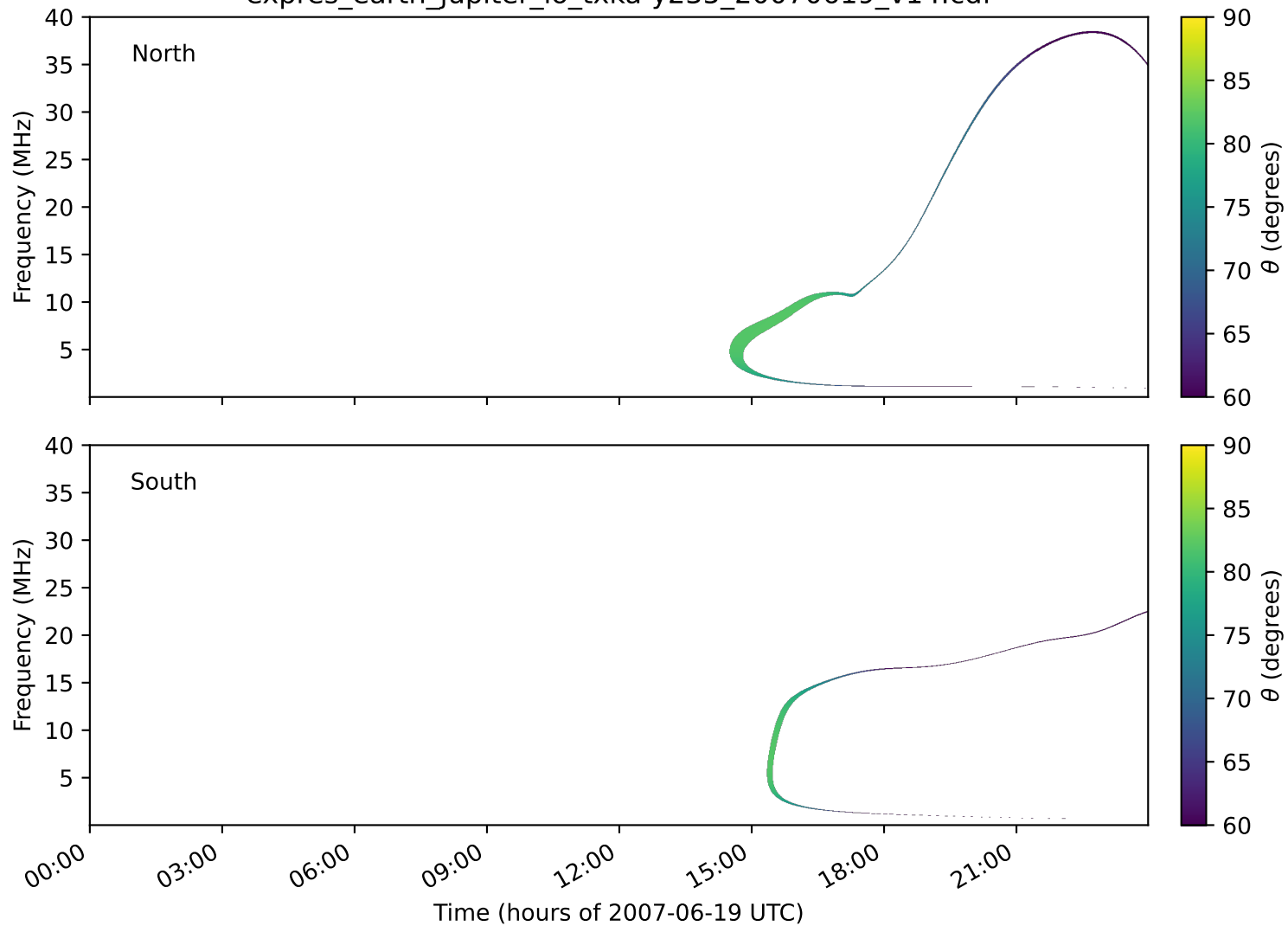
expres_earth_jupiter_io_txka-y235_20070619_v14.cdf
