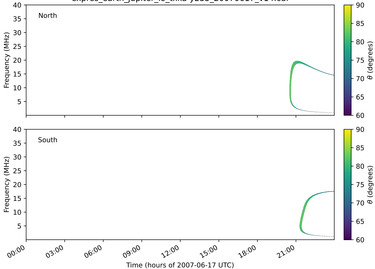
expres_earth_jupiter_io_txka-y235_20070617_v14.cdf
