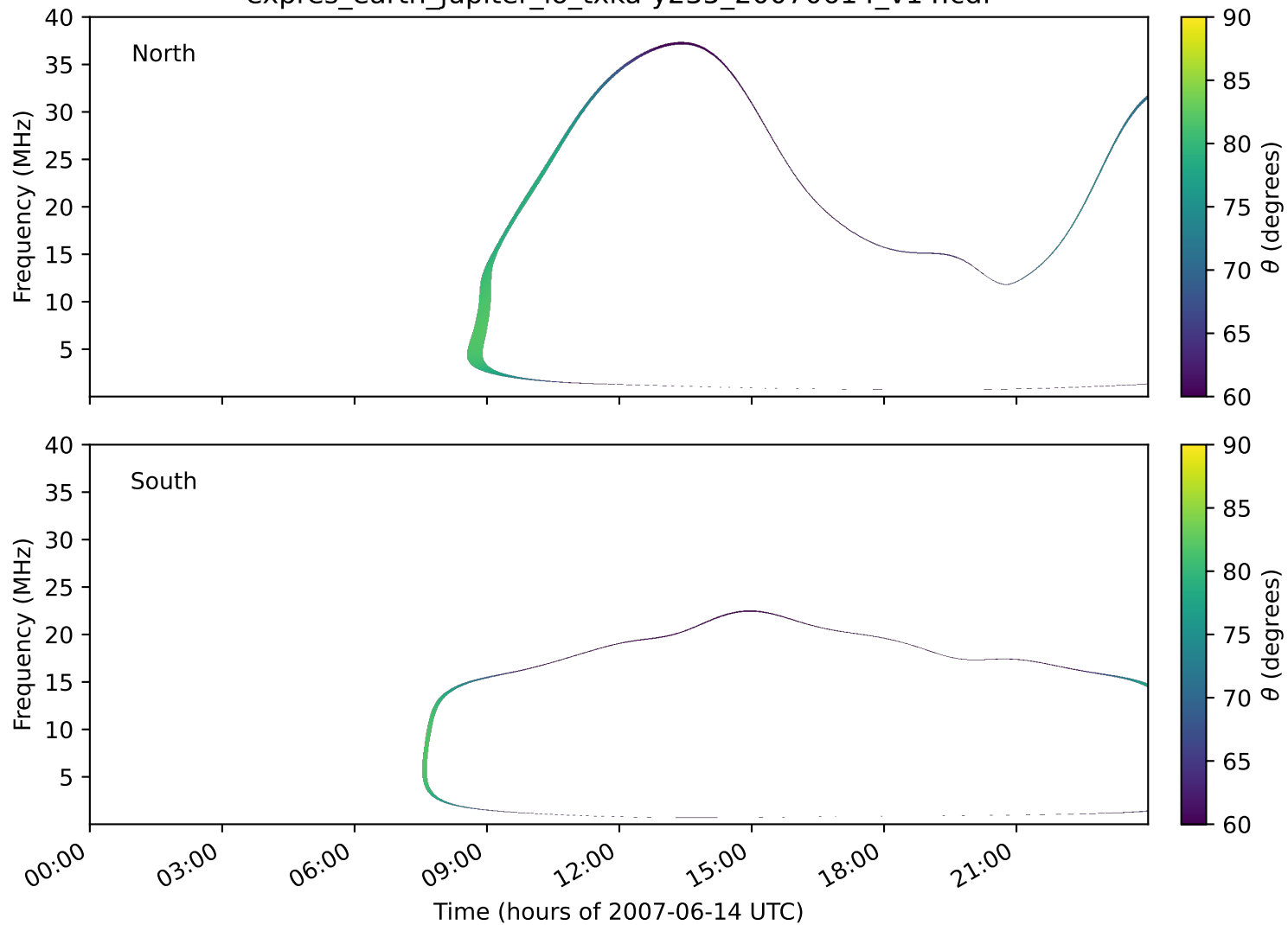
expres_earth_jupiter_io_txka-y235_20070614_v14.cdf
