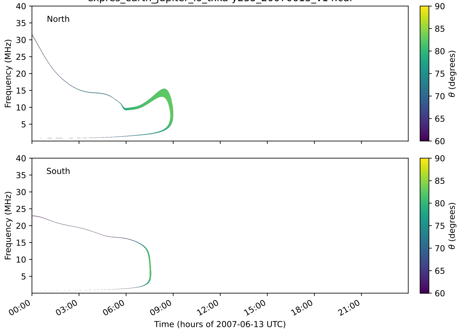
expres_earth_jupiter_io_txka-y235_20070613_v14.cdf
