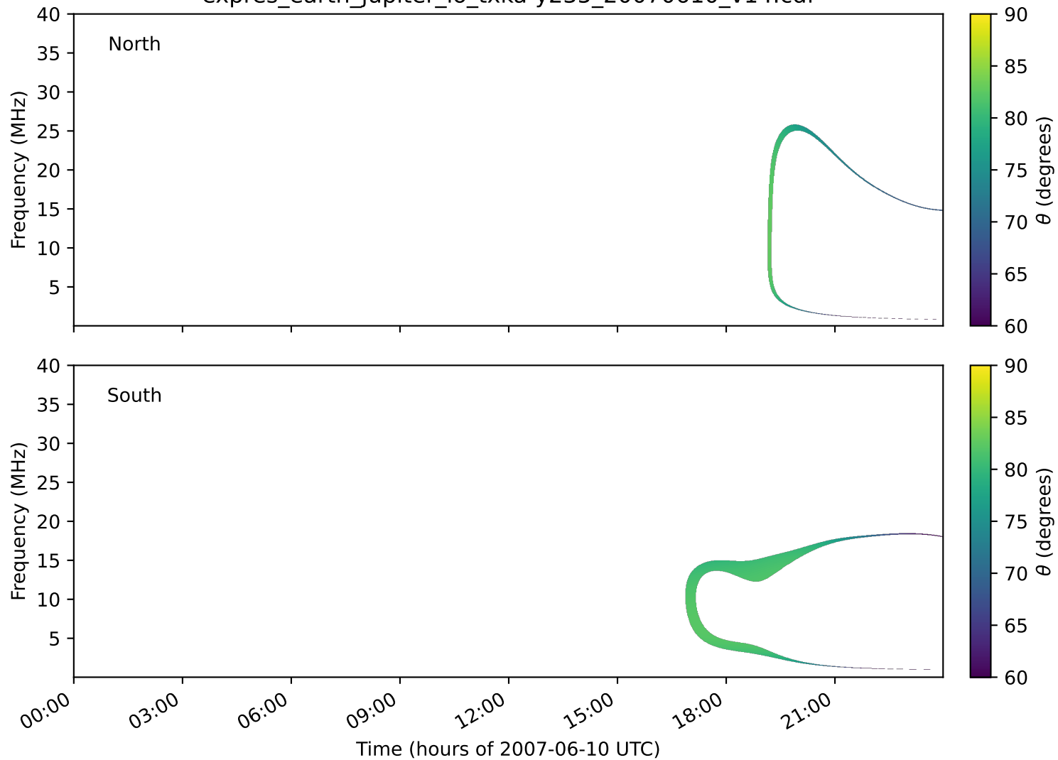
expres_earth_jupiter_io_txka-y235_20070610_v14.cdf
