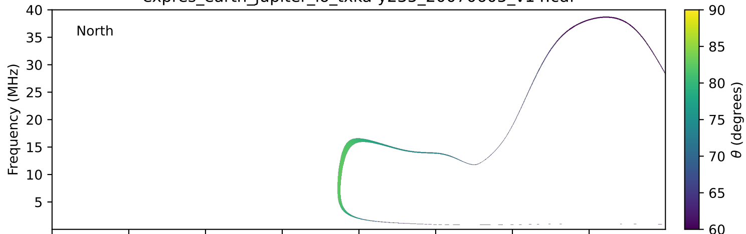
expres_earth_jupiter_io_txka-y235_20070605_v14.cdf
