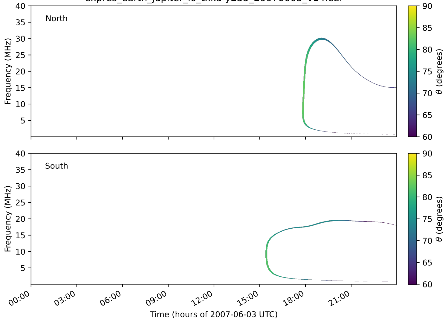
expres_earth_jupiter_io_txka-y235_20070603_v14.cdf
