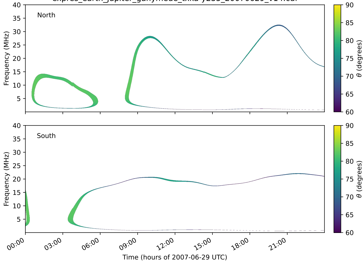
expres_earth_jupiter_ganymede_txka-y235_20070629_v14.cdf
