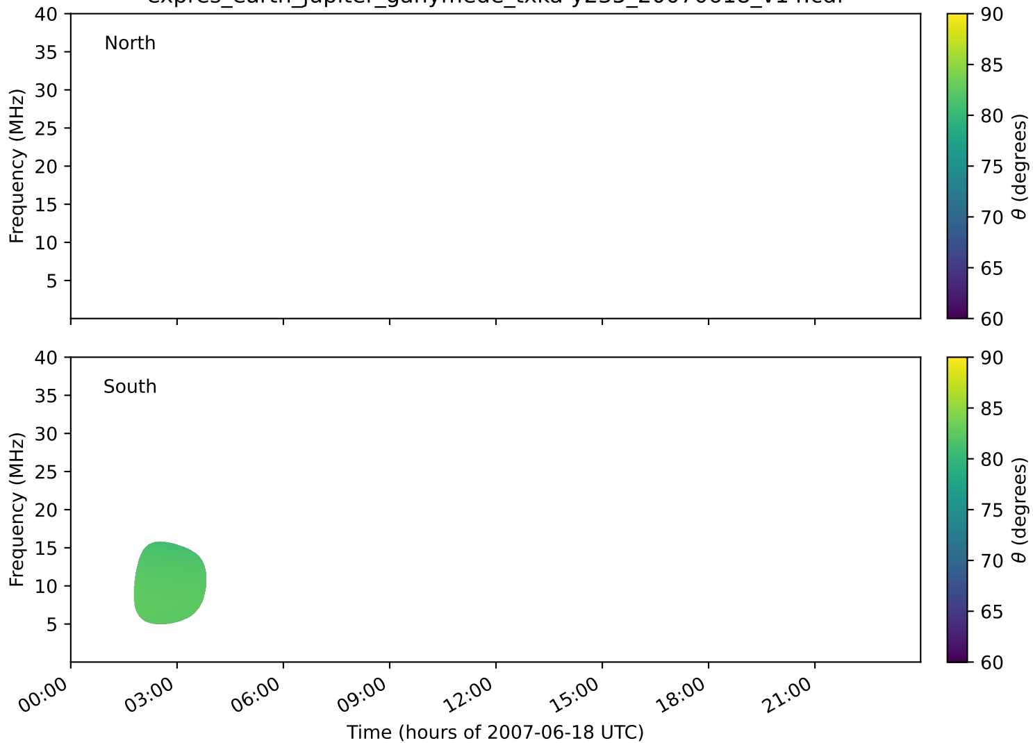
expres_earth_jupiter_ganymede_txka-y235_20070618_v14.cdf
