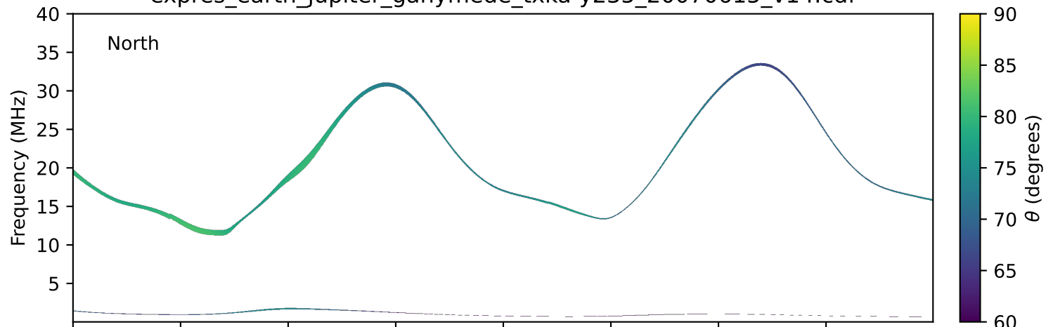
expres_earth_jupiter_ganymede_txka-y235_20070615_v14.cdf
