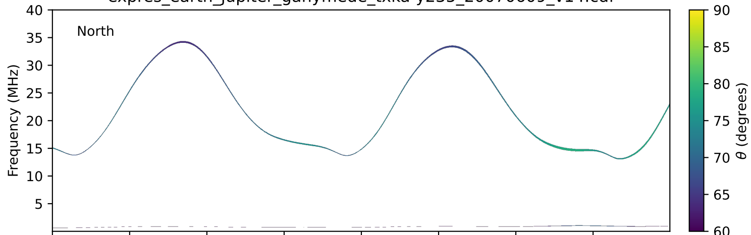
expres_earth_jupiter_ganymede_txka-y235_20070609_v14.cdf
