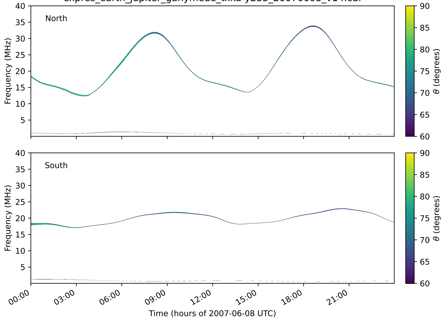
expres_earth_jupiter_ganymede_txka-y235_20070608_v14.cdf
