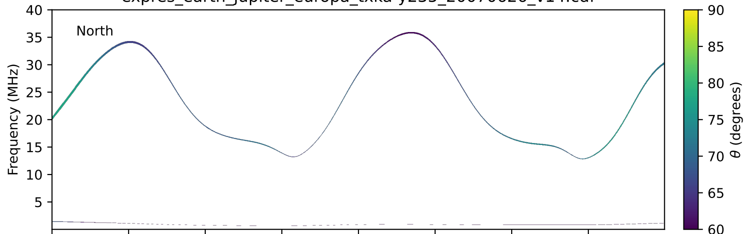
expres_earth_jupiter_europa_txka-y235_20070626_v14.cdf
