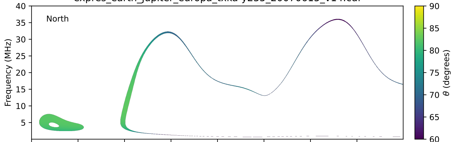
expres_earth_jupiter_europa_txka-y235_20070615_v14.cdf
