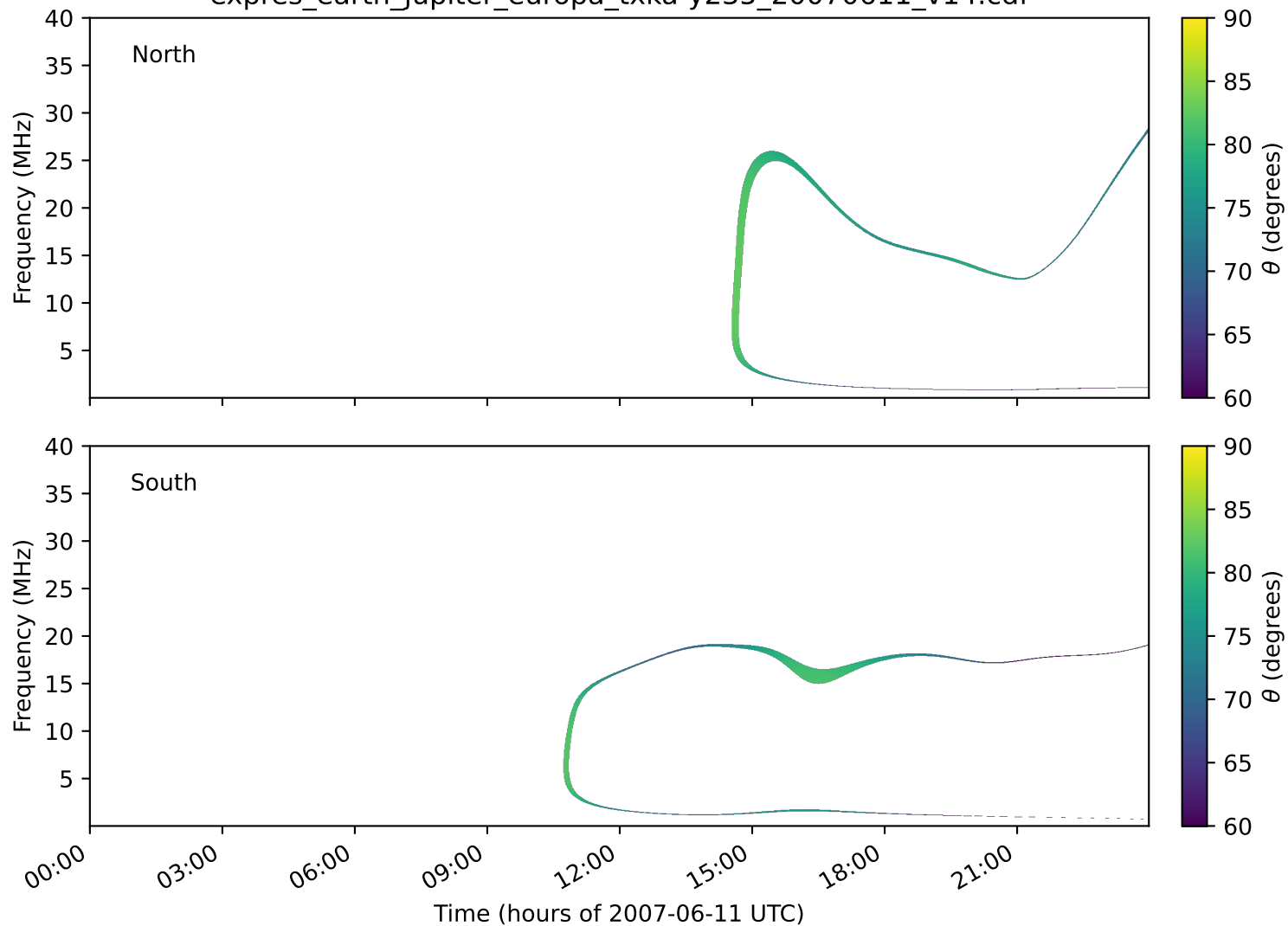
expres_earth_jupiter_europa_txka-y235_20070611_v14.cdf
