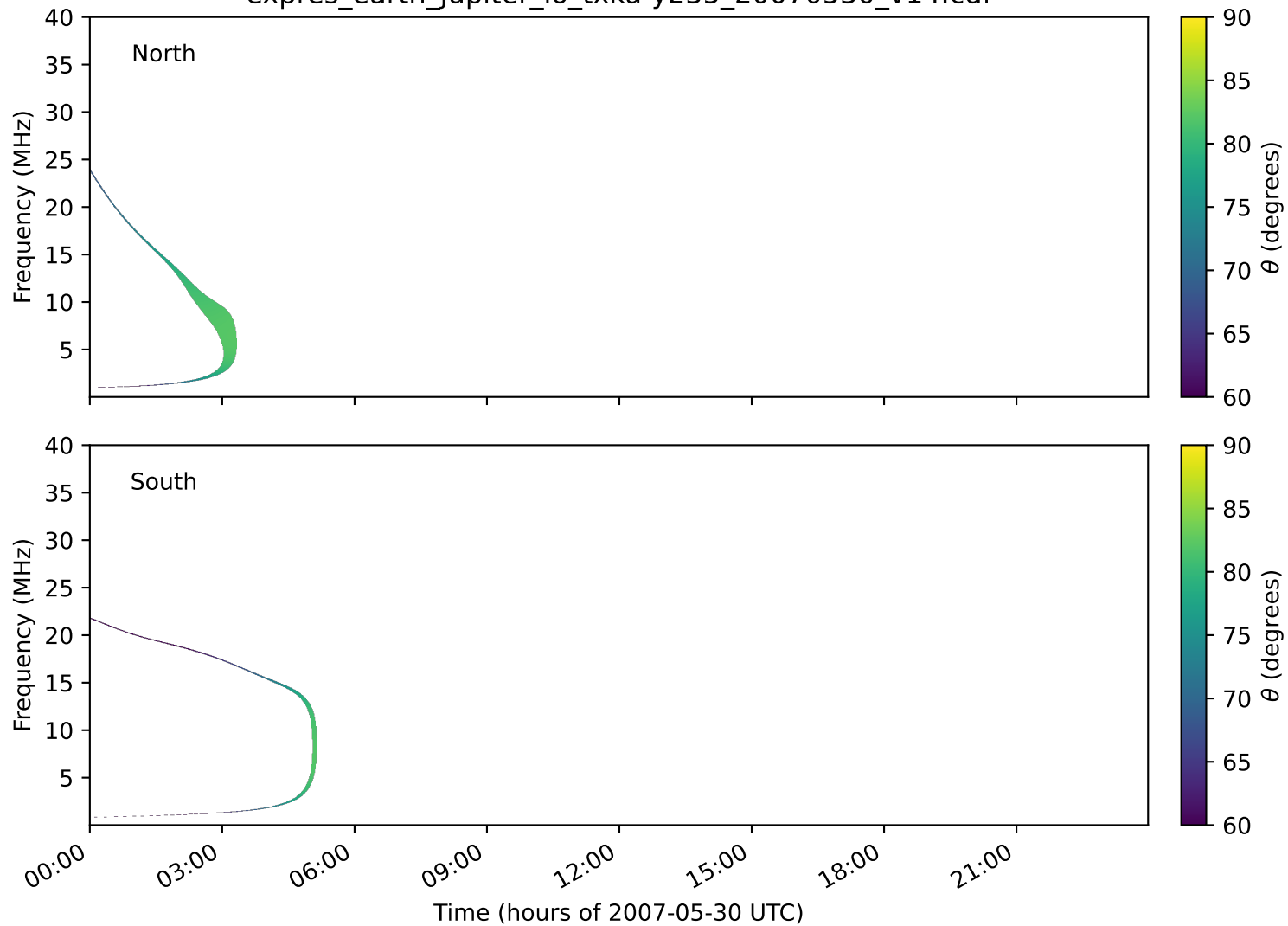
expres_earth_jupiter_io_txka-y235_20070530_v14.cdf
