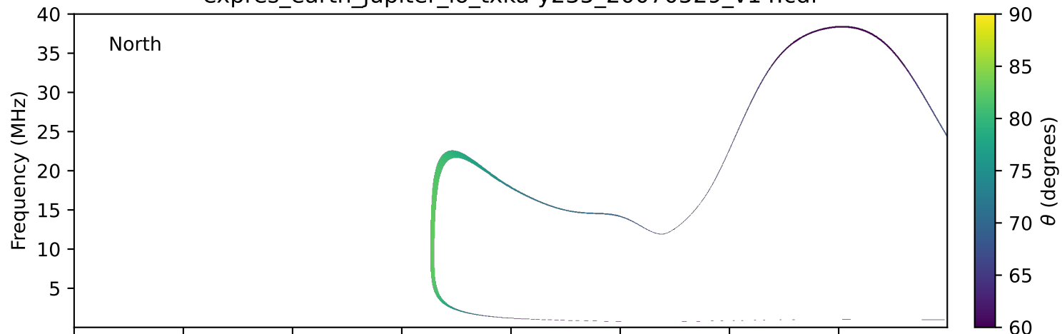
expres_earth_jupiter_io_txka-y235_20070529_v14.cdf
