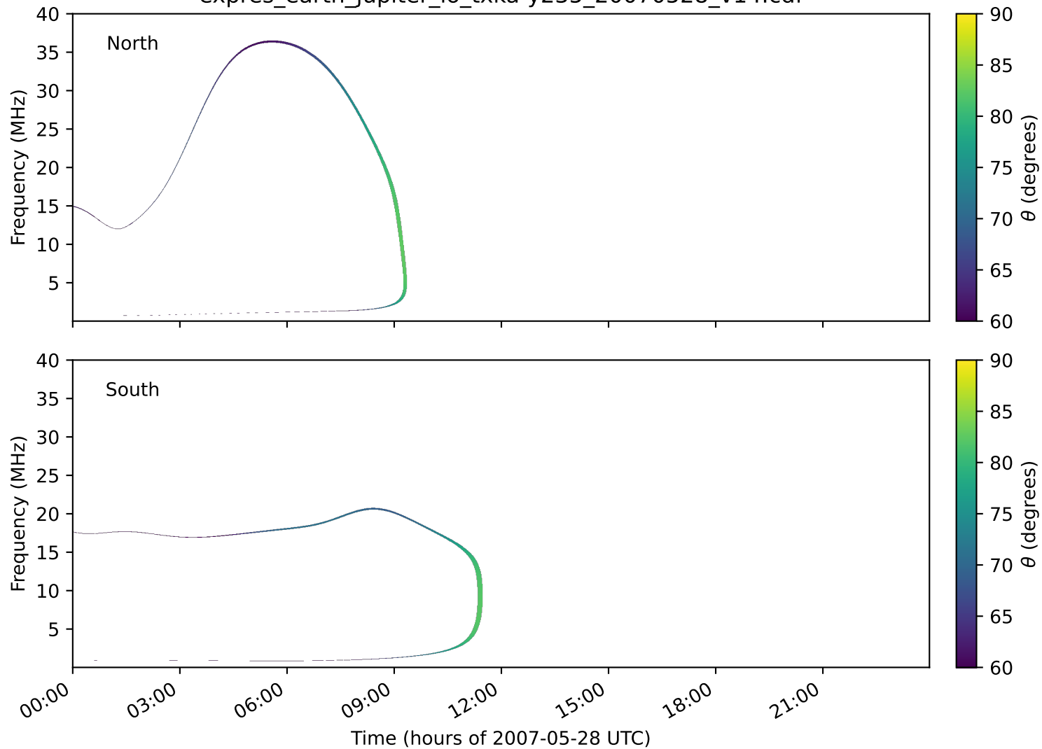
expres_earth_jupiter_io_txka-y235_20070528_v14.cdf
