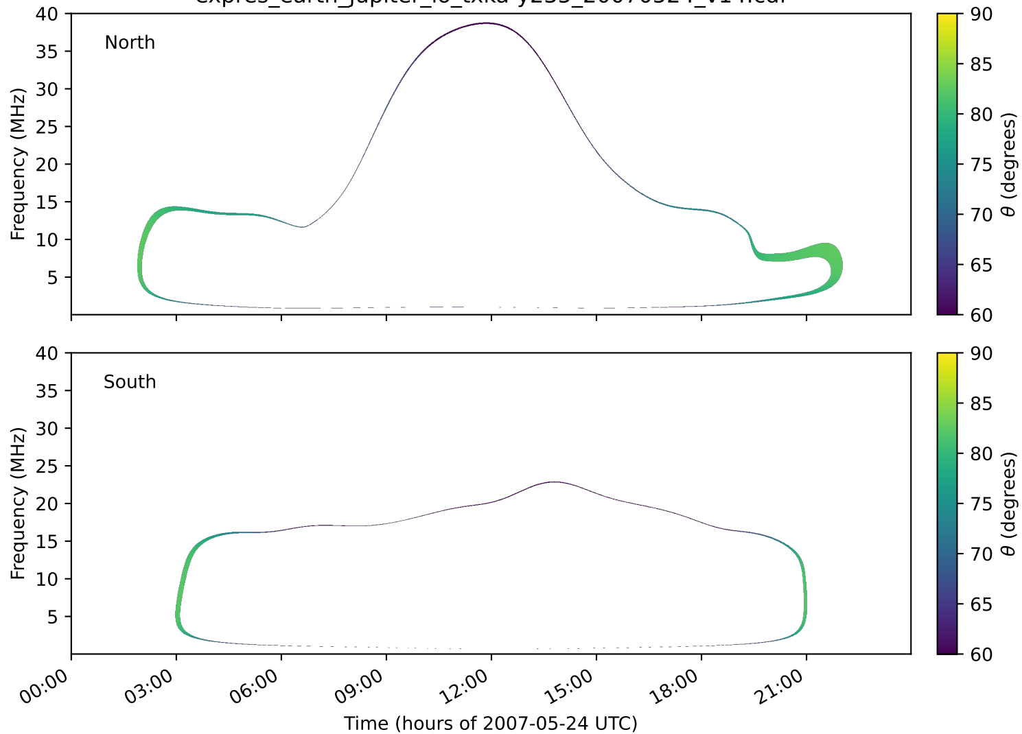
expres_earth_jupiter_io_txka-y235_20070524_v14.cdf
