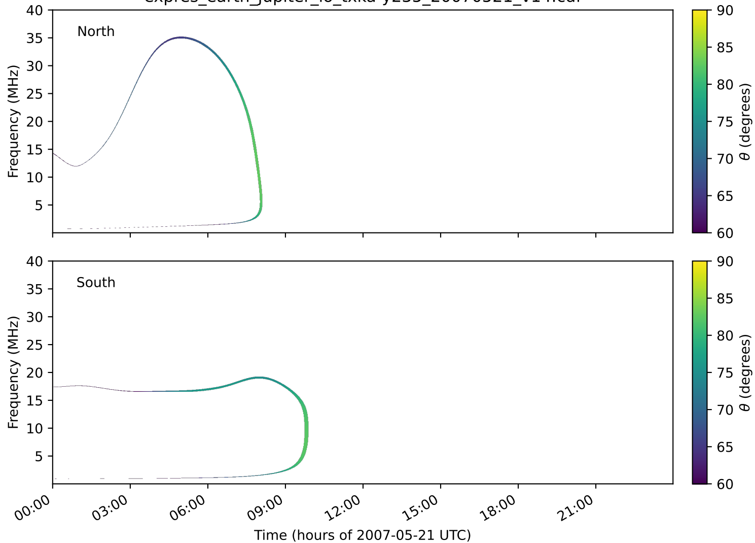
expres_earth_jupiter_io_txka-y235_20070521_v14.cdf
