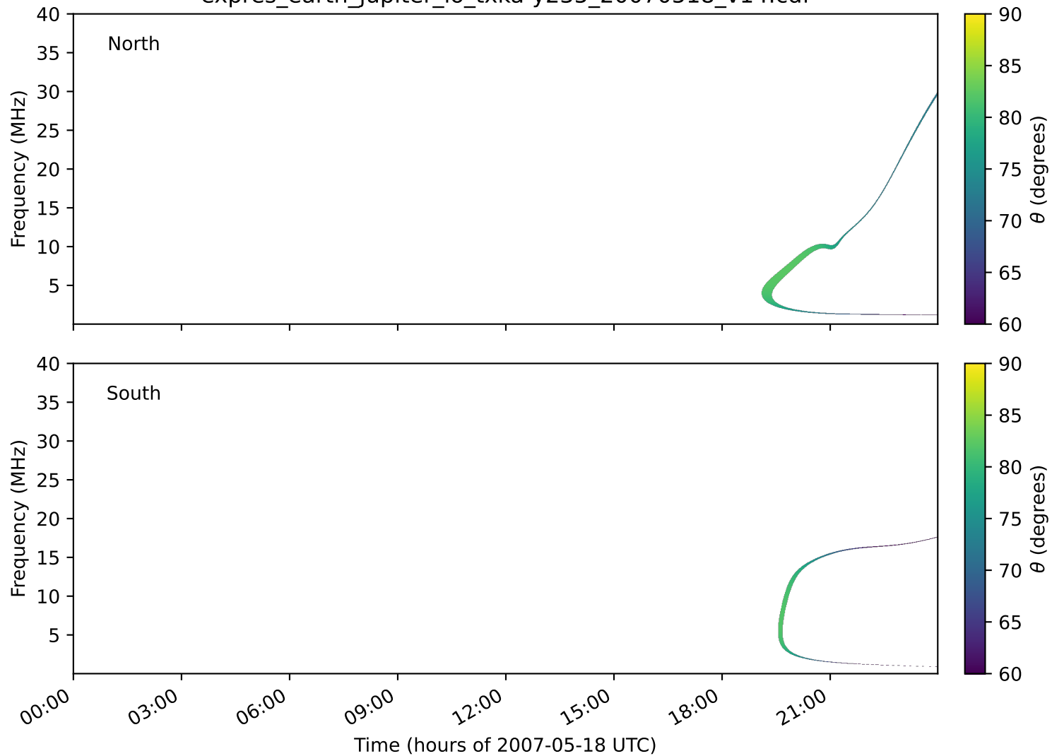
expres_earth_jupiter_io_txka-y235_20070518_v14.cdf
