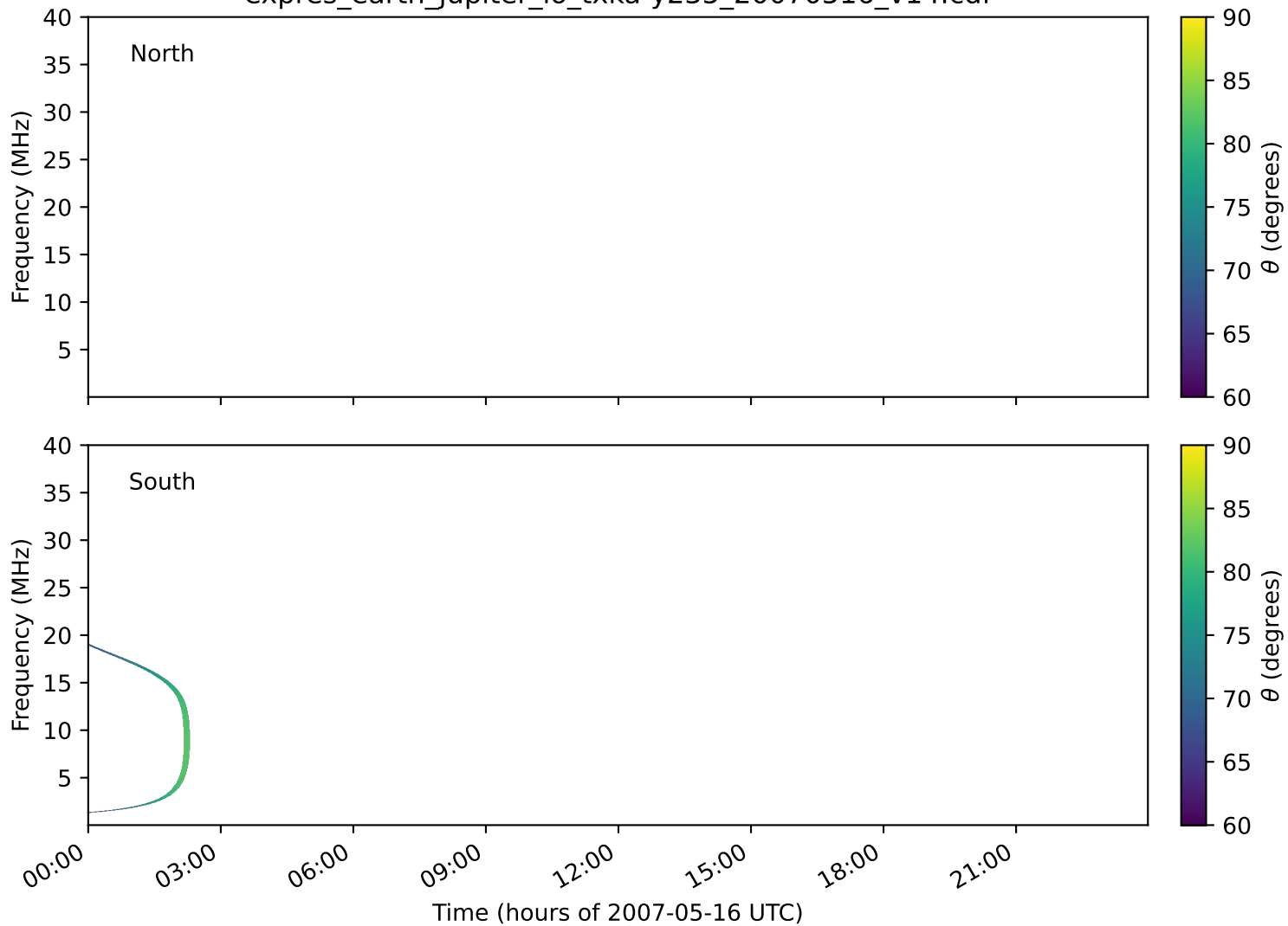
expres_earth_jupiter_io_txka-y235_20070516_v14.cdf
