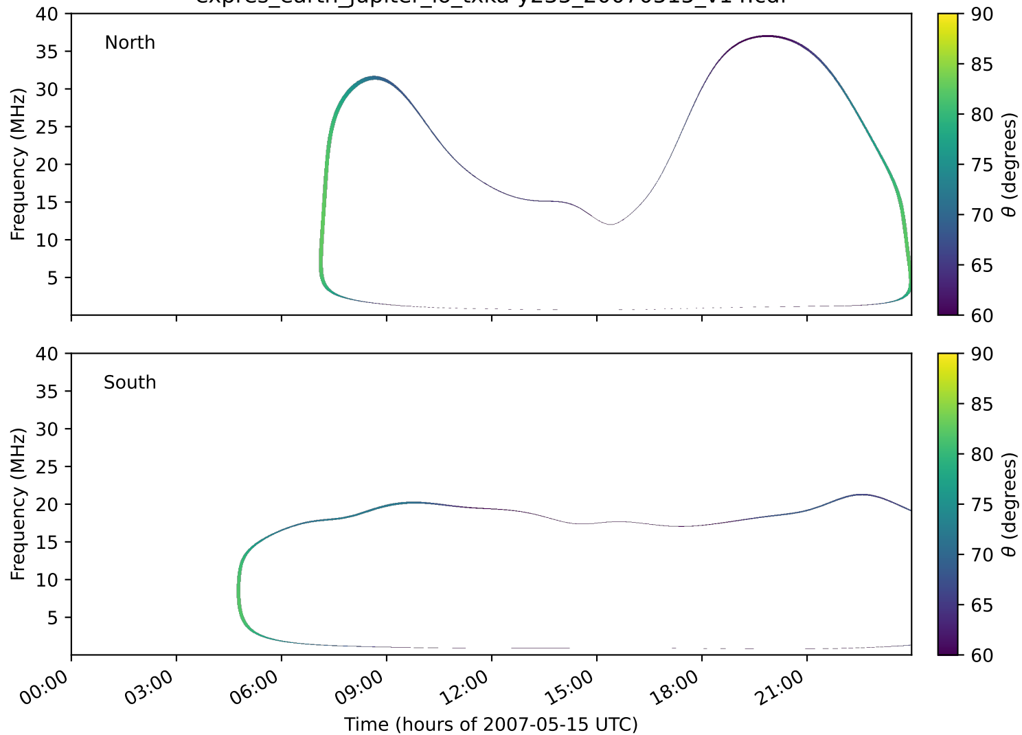
expres_earth_jupiter_io_txka-y235_20070515_v14.cdf
