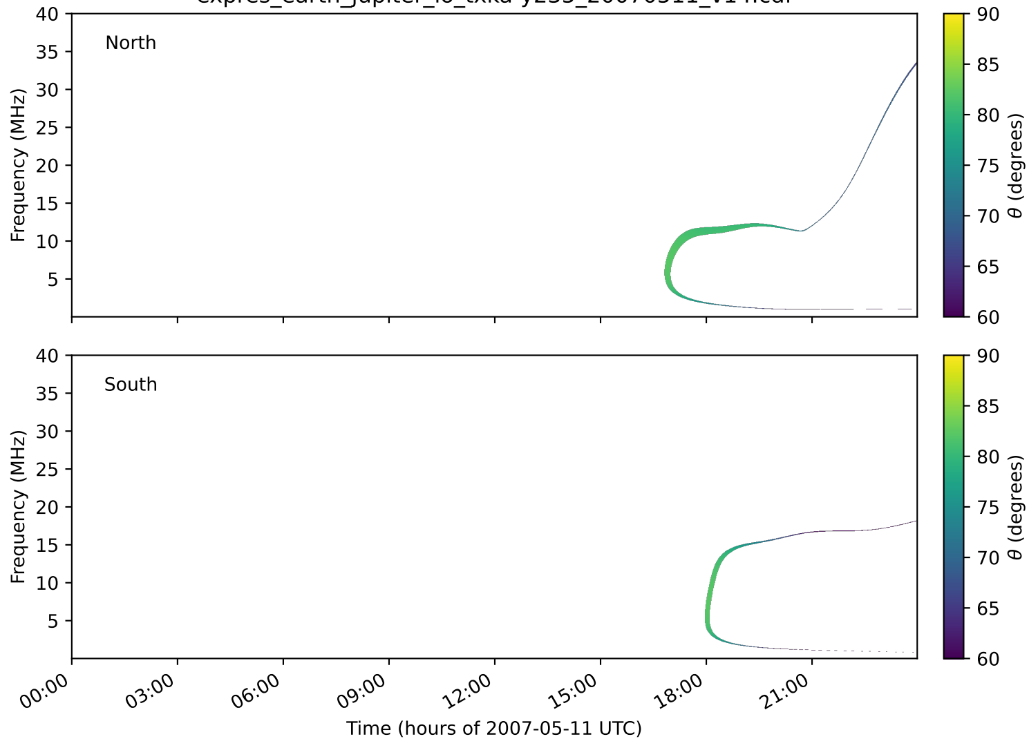
expres_earth_jupiter_io_txka-y235_20070511_v14.cdf
