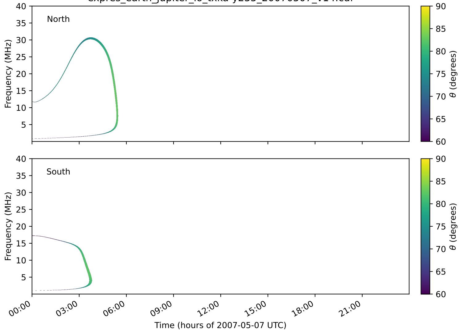
expres_earth_jupiter_io_txka-y235_20070507_v14.cdf
