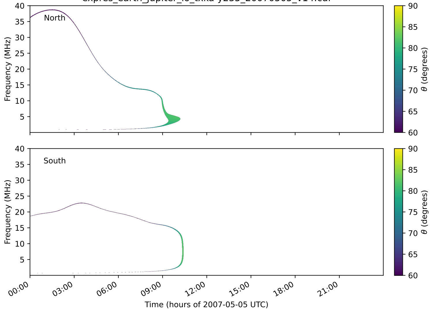
expres_earth_jupiter_io_txka-y235_20070505_v14.cdf
