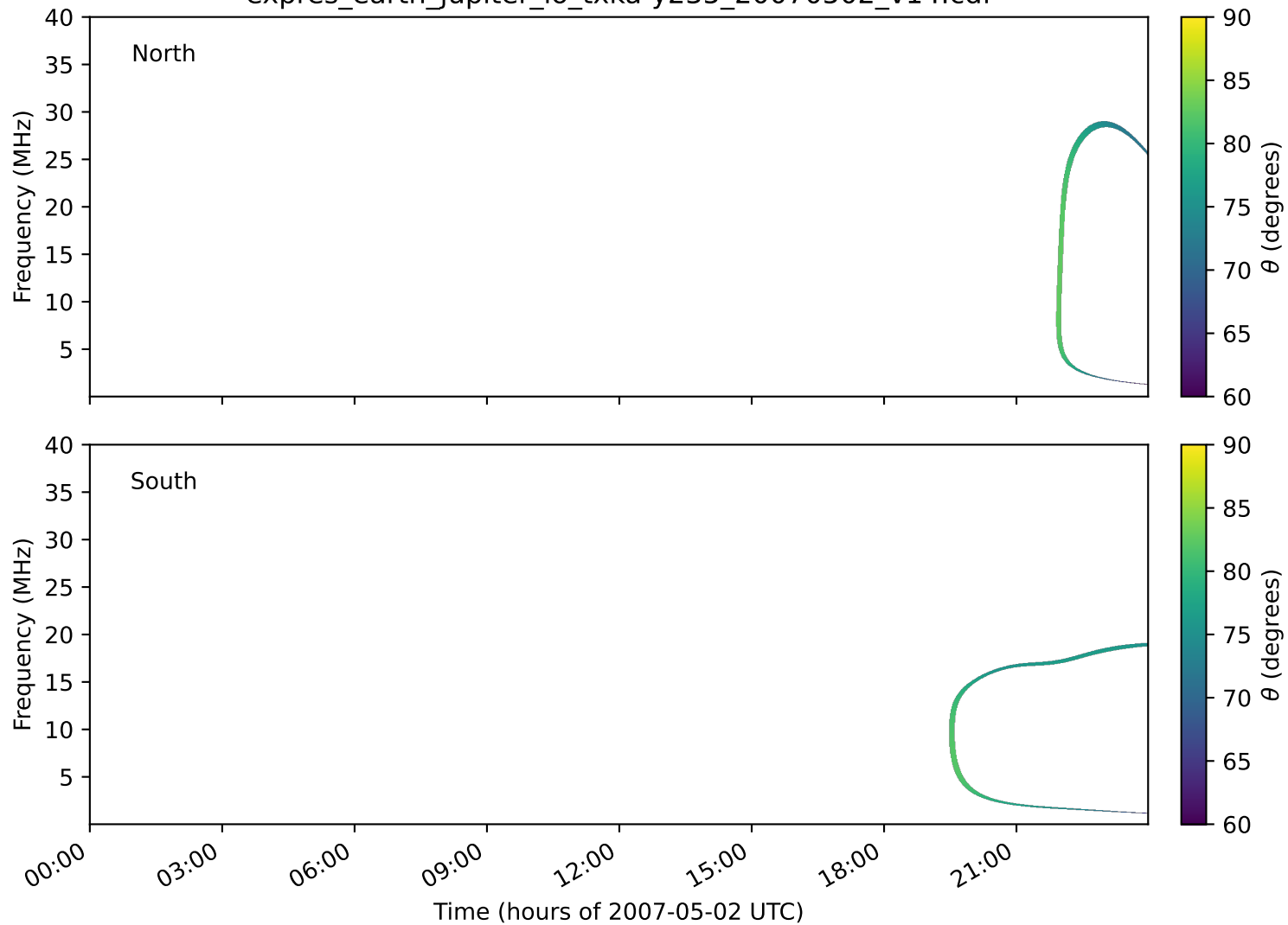
expres_earth_jupiter_io_txka-y235_20070502_v14.cdf
