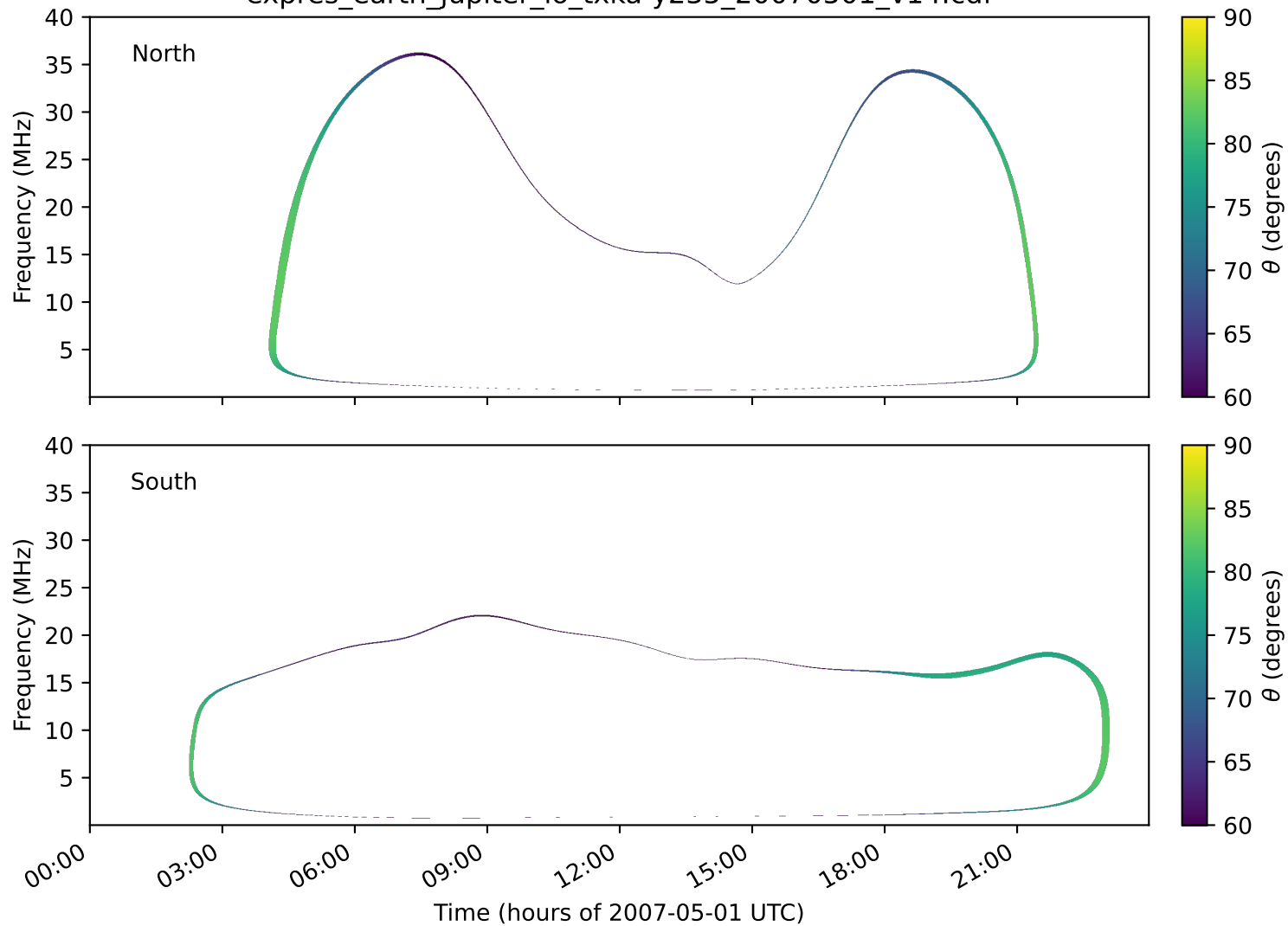
expres_earth_jupiter_io_txka-y235_20070501_v14.cdf
