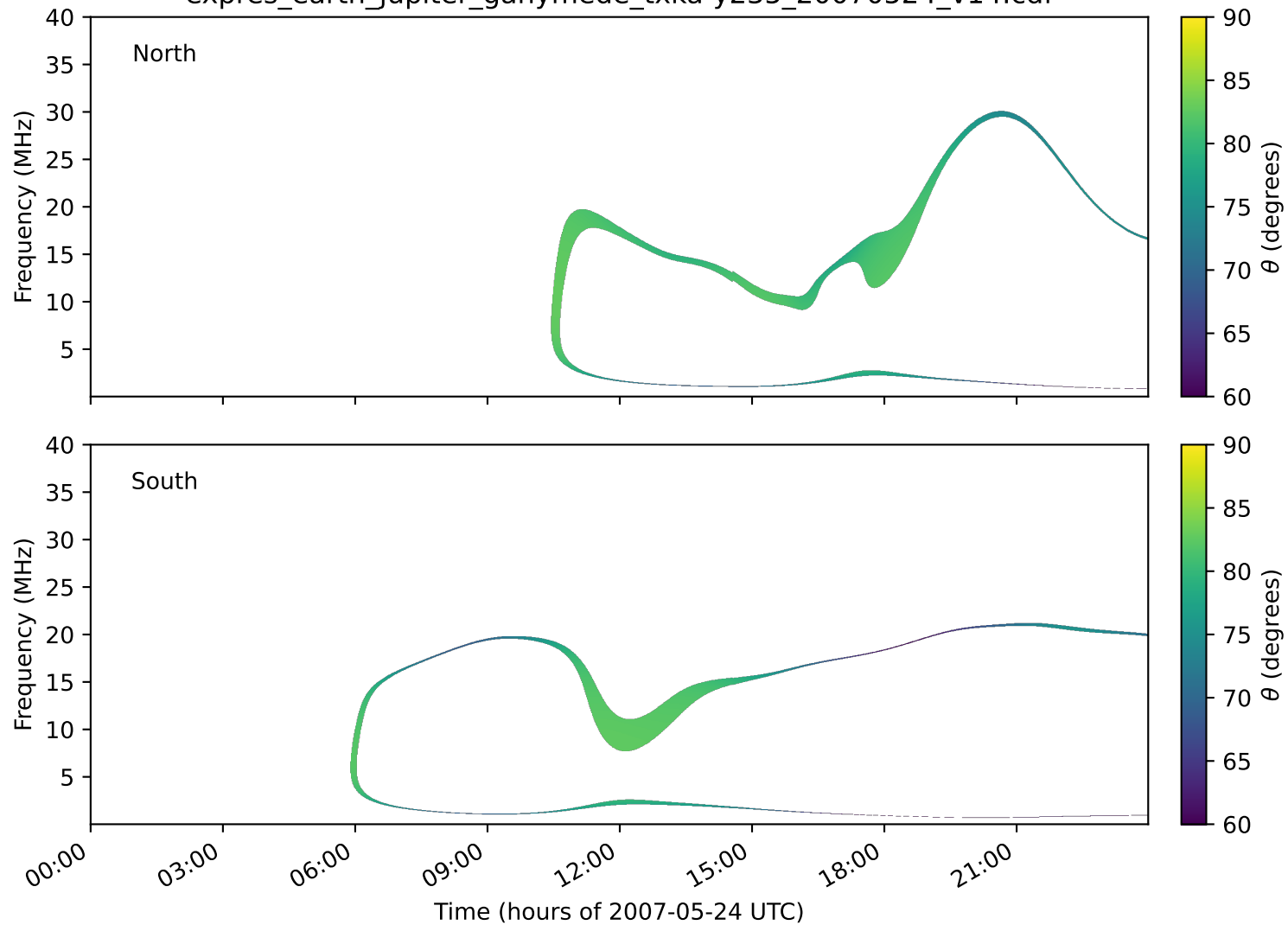
expres_earth_jupiter_ganymede_txka-y235_20070524_v14.cdf
