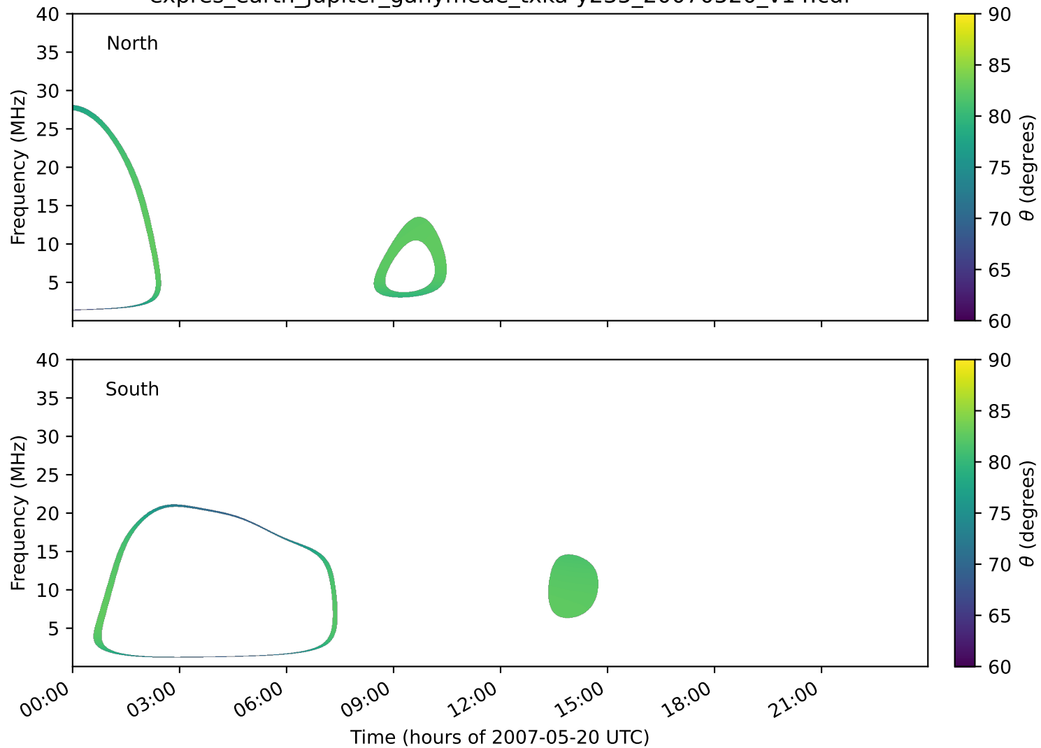
expres_earth_jupiter_ganymede_txka-y235_20070520_v14.cdf
