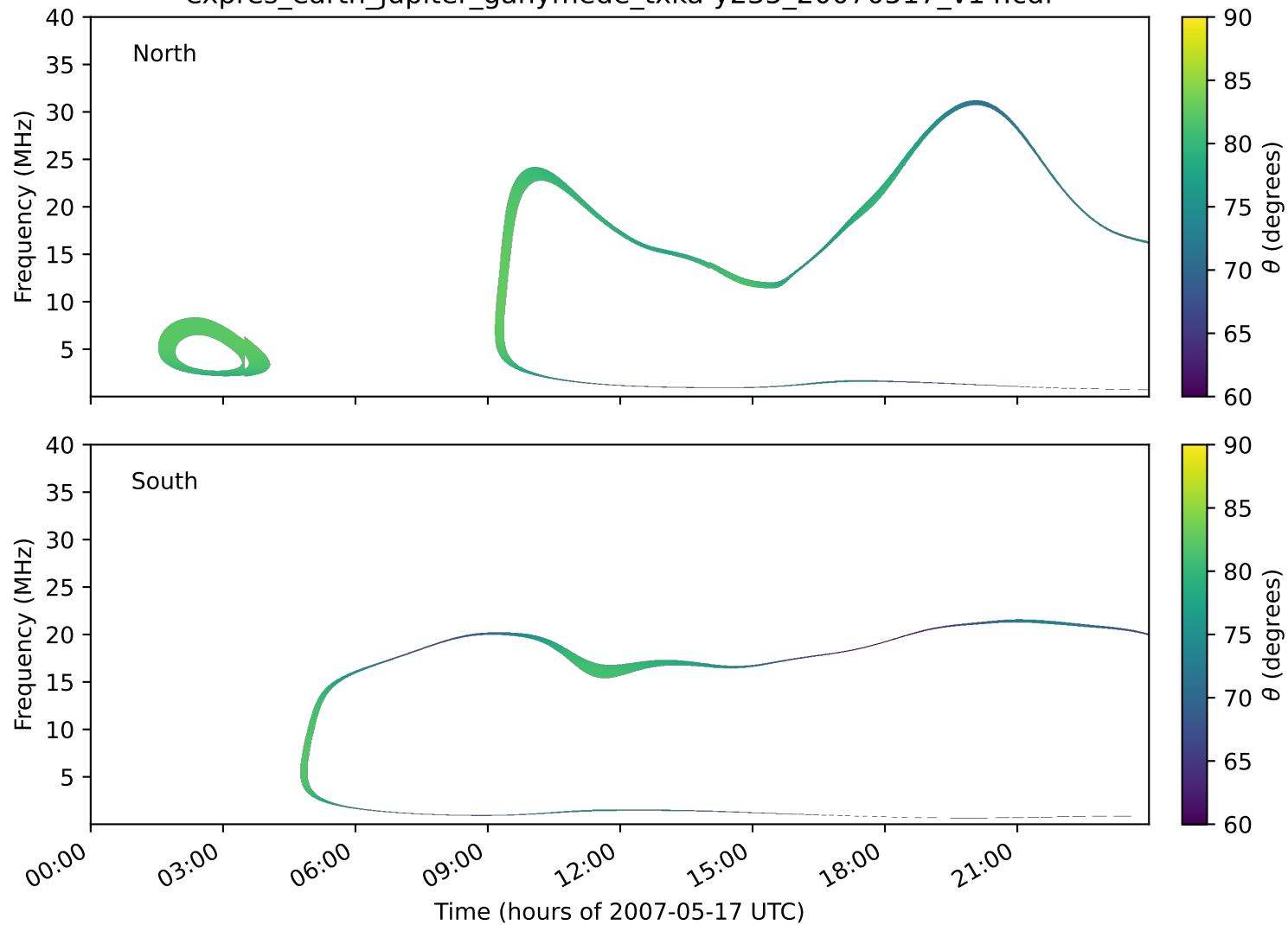
expres_earth_jupiter_ganymede_txka-y235_20070517_v14.cdf
