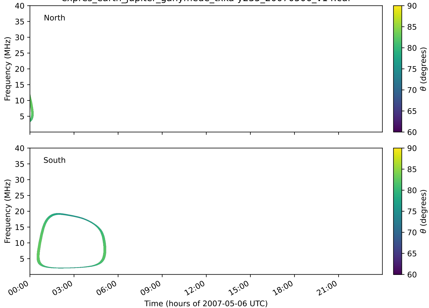
expres_earth_jupiter_ganymede_txka-y235_20070506_v14.cdf
