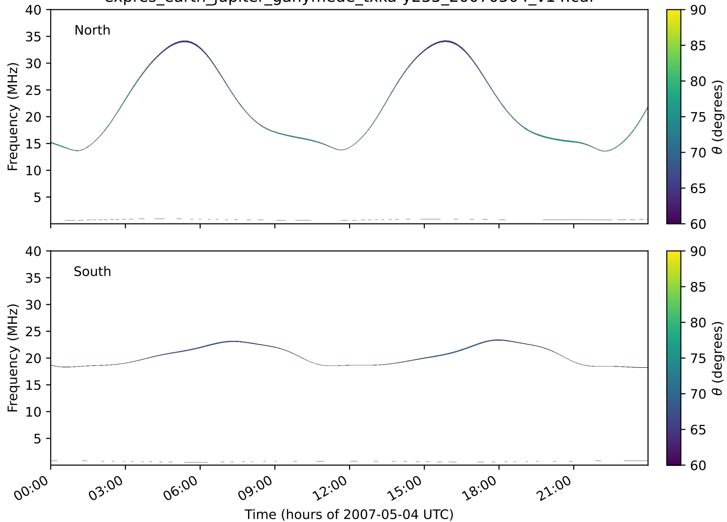
expres_earth_jupiter_ganymede_txka-y235_20070504_v14.cdf
