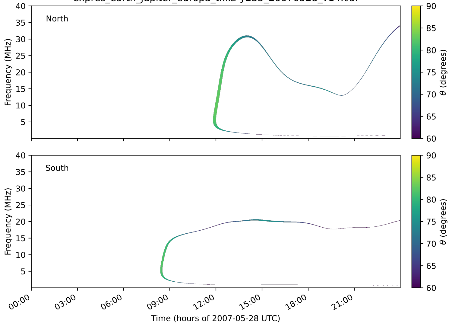
expres_earth_jupiter_europa_txka-y235_20070528_v14.cdf
