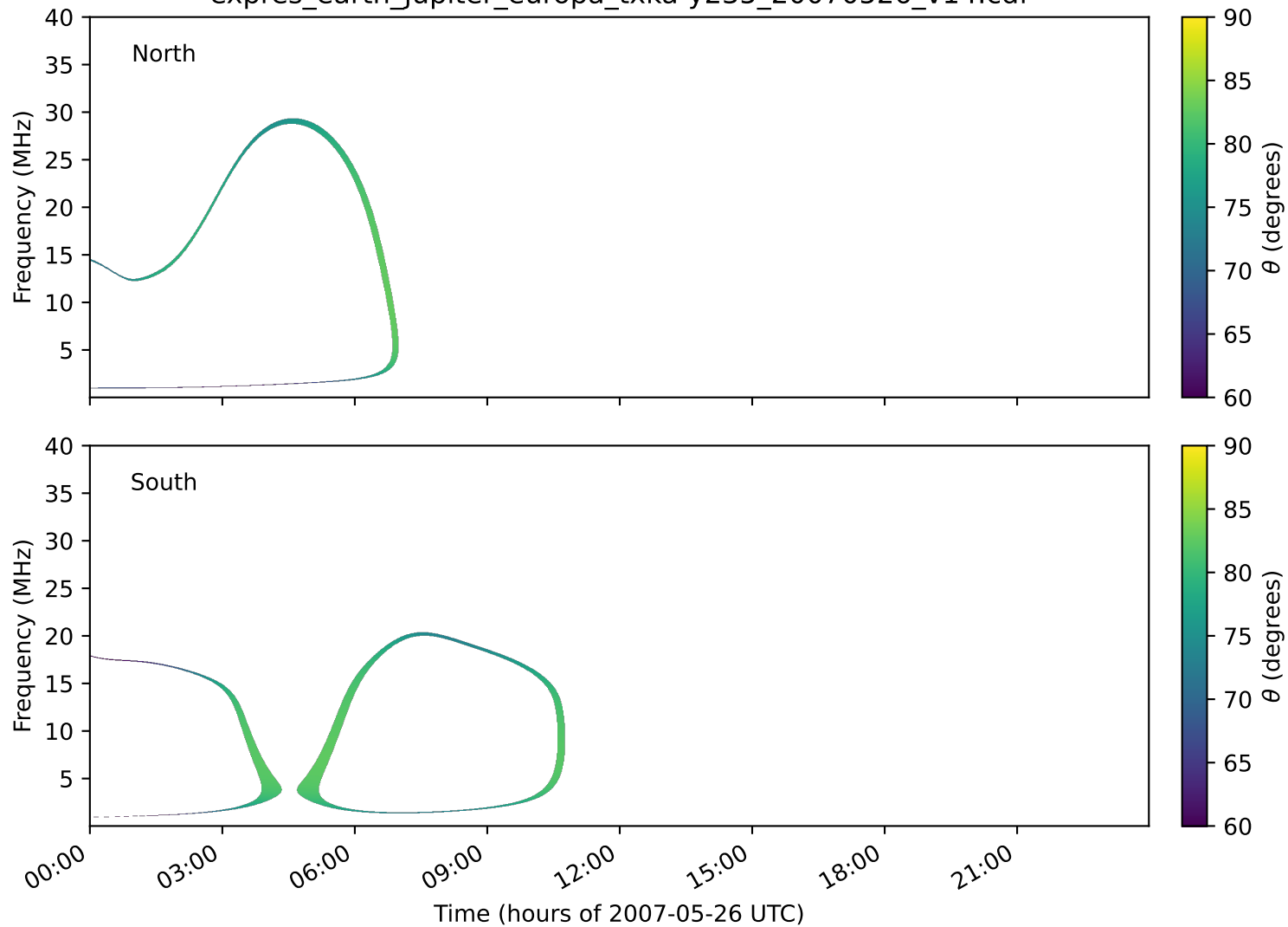
expres_earth_jupiter_europa_txka-y235_20070526_v14.cdf
