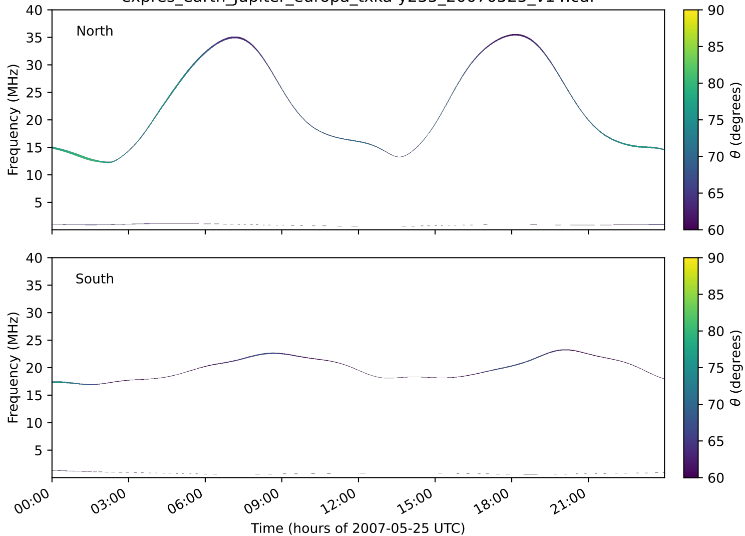
expres_earth_jupiter_europa_txka-y235_20070525_v14.cdf
